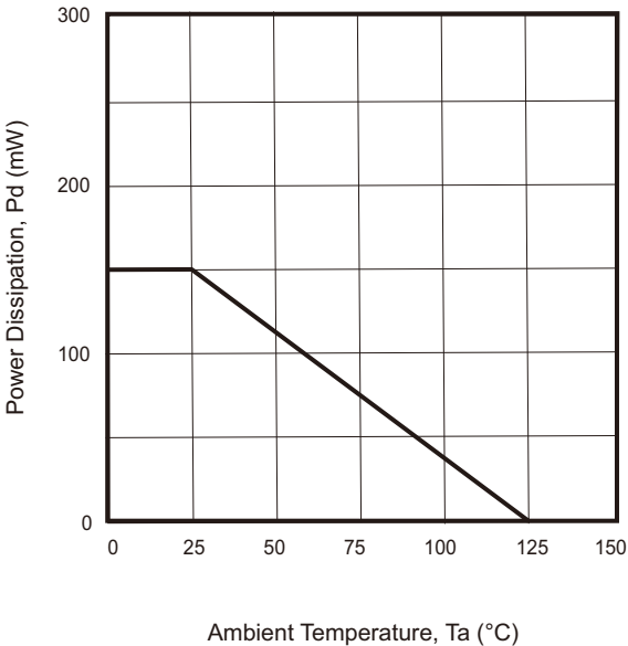
Fig.2 - Derating Curve
